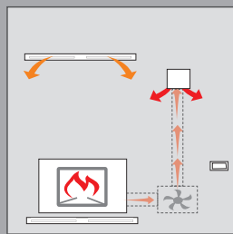
KIT AIR DIFFUSER
